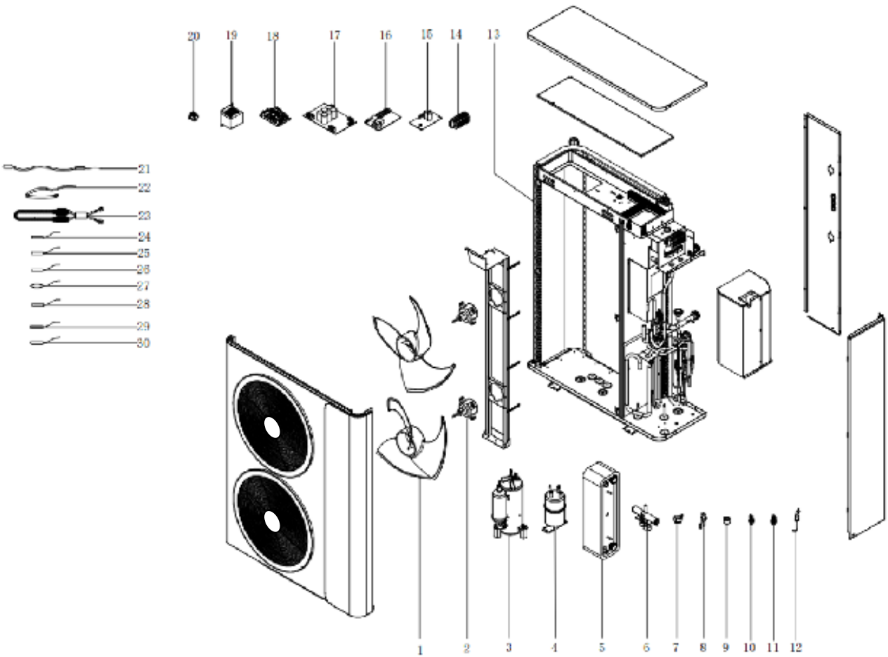
CubeHPM 15
