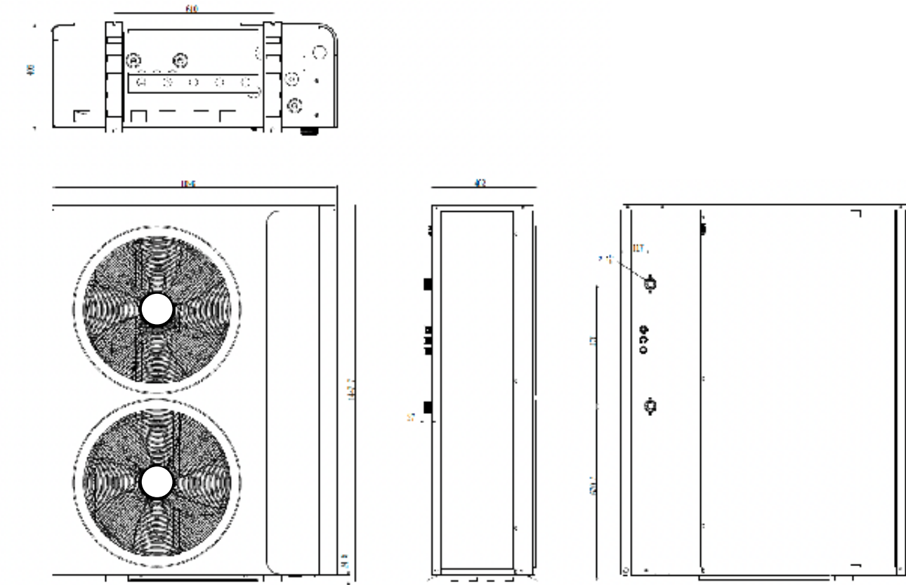
Cube HPM15
