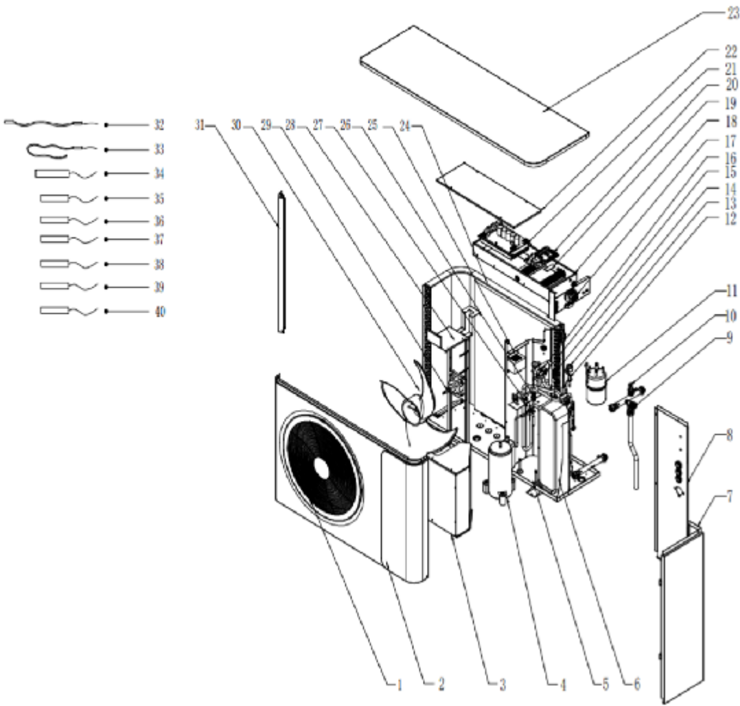
CubeHPM 12
